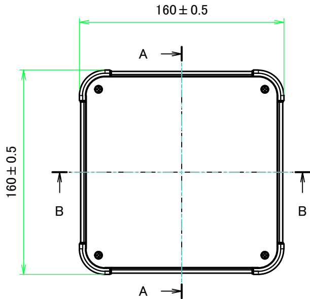
E view
